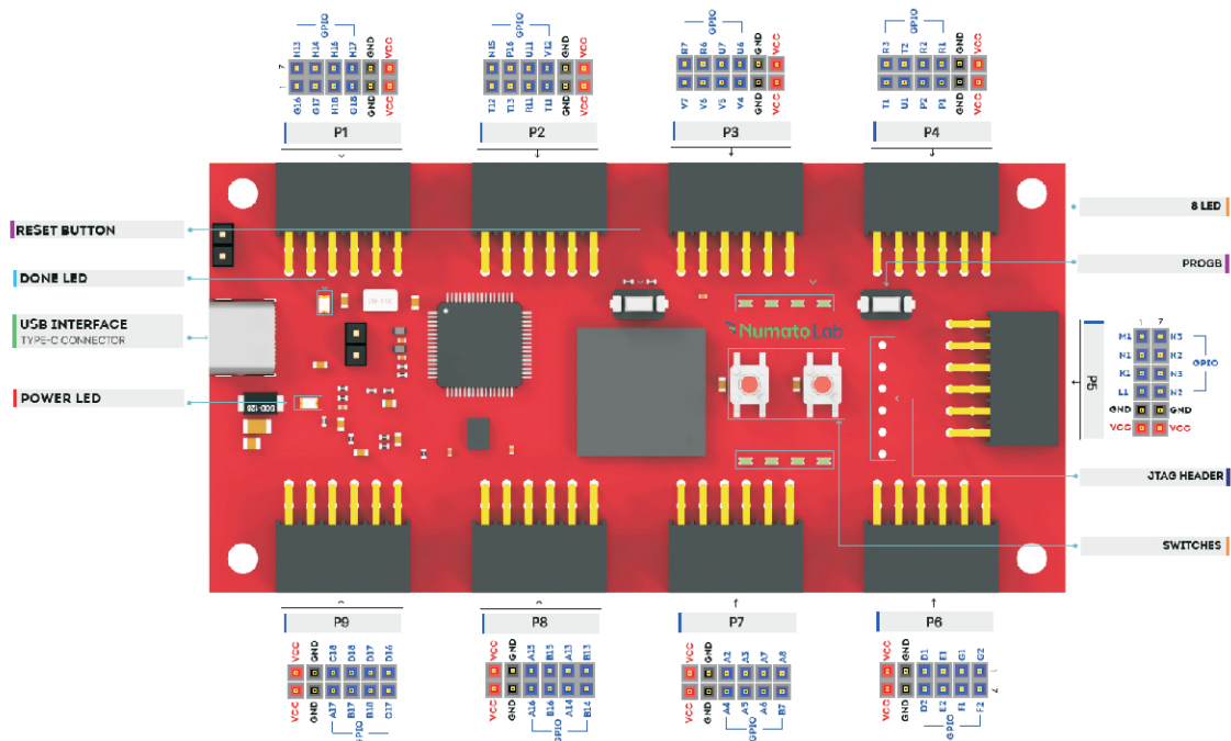
Wiring Diagram
