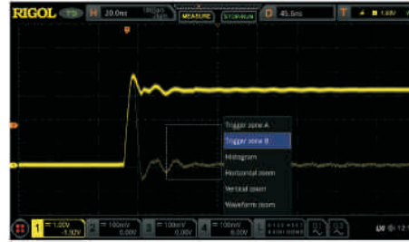
Draw a rectangle on the transient exception signal and select Trigger zone A.
