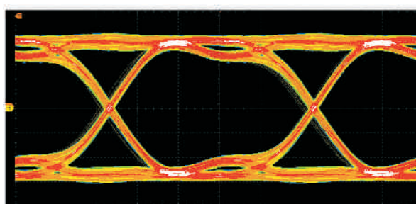
Use the 750 MHz bandwidth and 1.5 GHz bandwidth model respectively to perform eye measurement on the 1 Gb/s signal.
