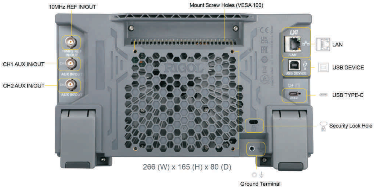
Ground Terminal
