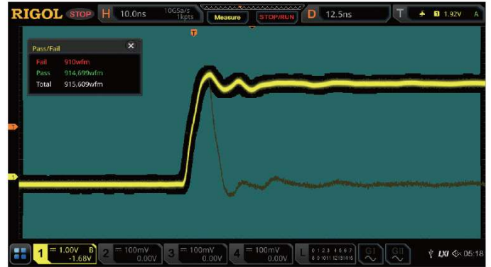
The Pass/Fail test function can quickly make a statistics on the occurrence probability of the signal exceptions.
