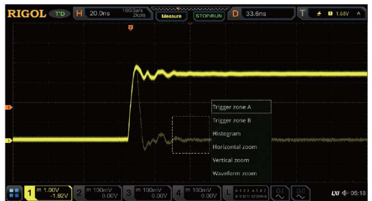
Draw a rectangle on the transient exception signal and select Trigger zone A.
