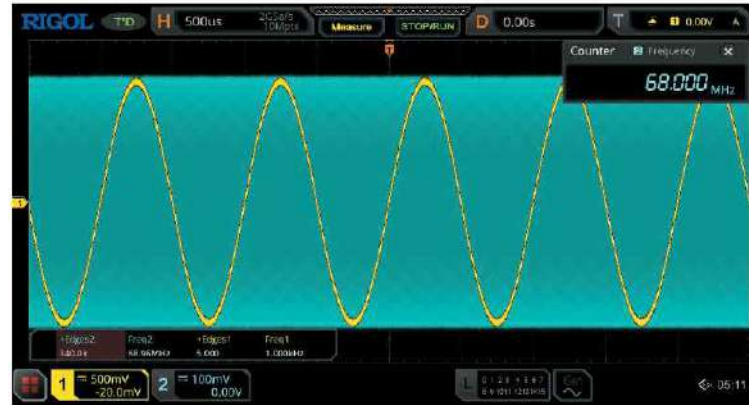
Observe and accurately measure two signals with great frequency deviations. The full-memory hardware measurement can measure accurate frequency value of the waveforms with 340k rising edges.
