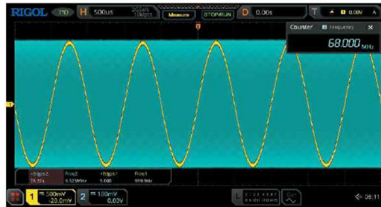
The ordinary 1 Mpts software measurement can no longer measure the accurate frequency of the high-frequency signal.
